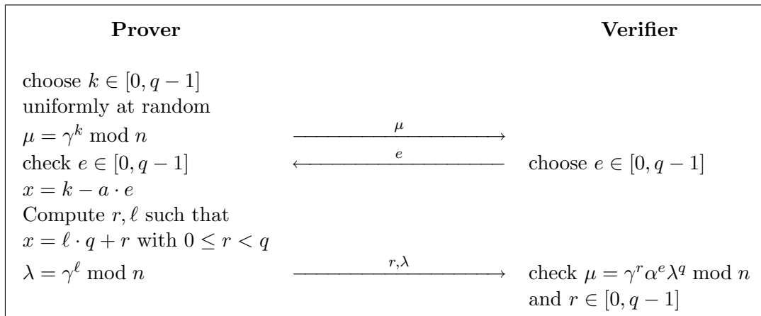
Figure 2: The RDSA identification scheme
